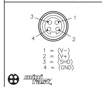
FEMALE END VIEW (J1-J4)
